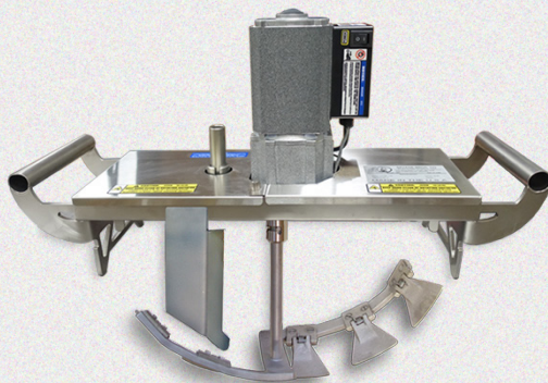
Portable Agitator
